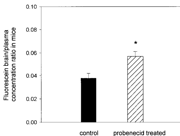
FIG. 5. The effect of probenecid on the brain distribution of fluorescein in wild-type FVB mice. Each value represents the mean \pm SE ( n = 6 ). * P < 0.01 , significantly different from the value of the corresponding control.
