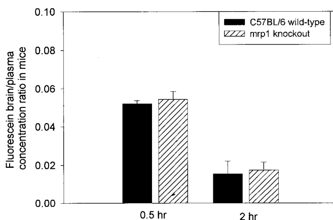
FIG. 4. The fluorescein brain/plasma concentration ratio in wild-type and mrp1(–/–) mice. Each value represents the mean \pm SE ( n = 4 ).
